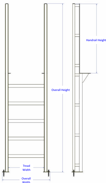
Vertical Ladder
