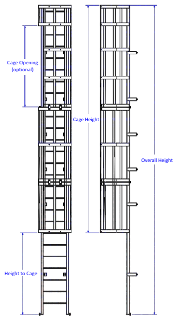
Caged Ladder
